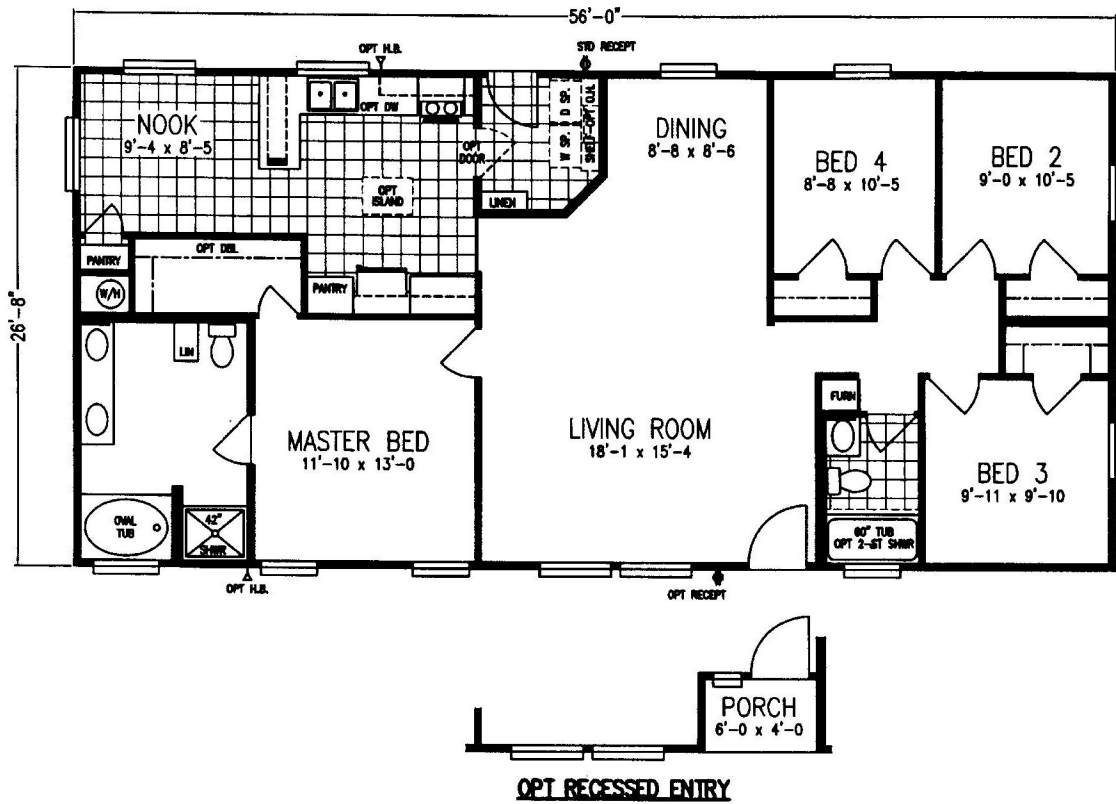
MODEL 568A APPROX. 1493 SQ. FT. 4 BEDROOM, 2 BATH
