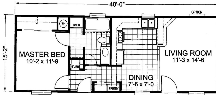
MODEL 406A APPROX. 607 SQ. FT. 1 BEDROOM, 1 BATH
